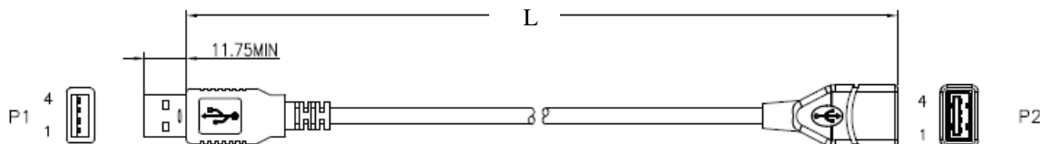
Outline Drawing (units mm)
