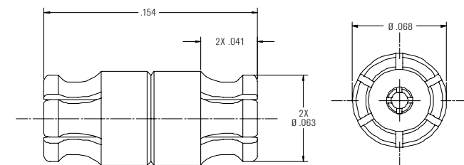
WMP® Female to WMP® Female Bullet / WP101-3CC
