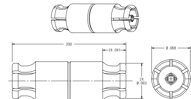
WMP® Female to WMP® Female Bullet / WP101-2CC
