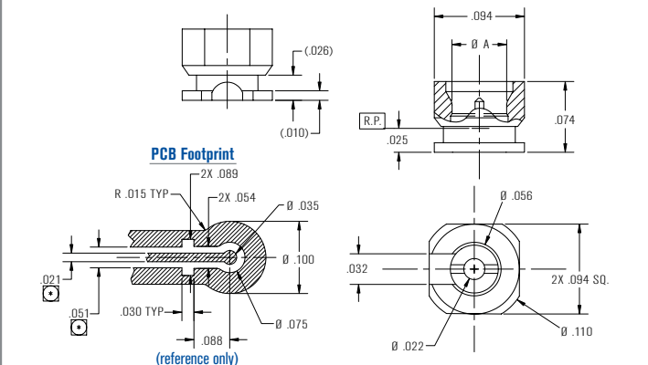
WMP® Male Straight Surface Mount / WP350
